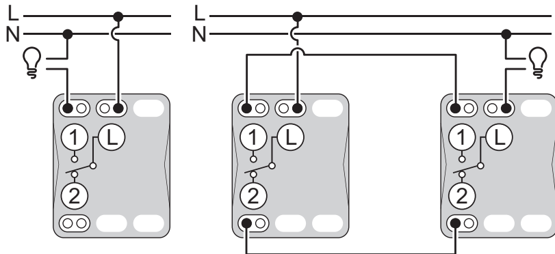
On/Off circuit
